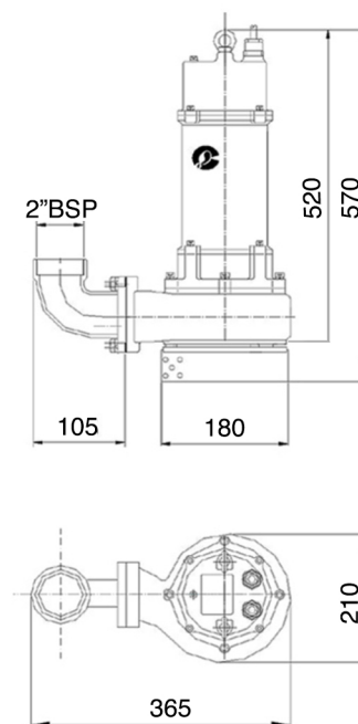
Pump Dimensions
